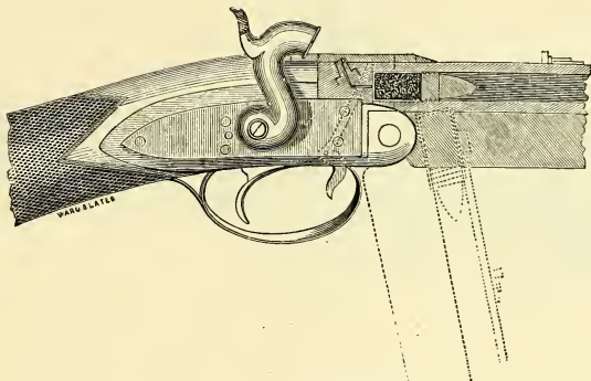
Gilbert Smith's American Carbine.
